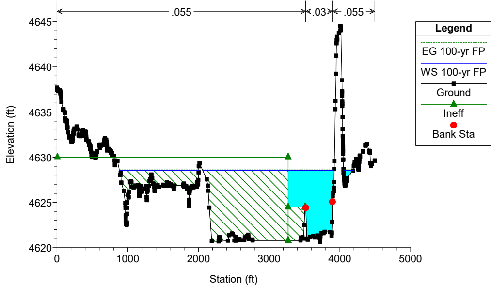
KCC-Lompa Ranch East_EOC Plan: KCC-Proposed Geom: Proposed Conditions Geometry Flow: FEMA Effective Flows River = KingsCynCreek Reach = Reach1 RS = 4309.763
