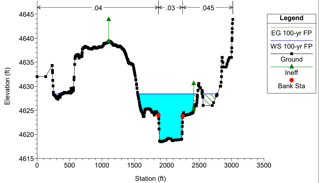
KCC-Lompa Ranch East_EOC Plan: KCC-Proposed Geom: Proposed Conditions Geometry Flow: FEMA Effective Flows River = KingsCynCreek Reach = Reach1 RS = 3923.687
