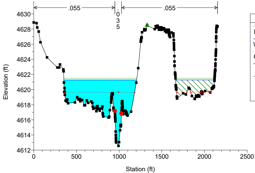
KCC-Lompa Ranch East_EOC Plan: KCC-Proposed Geom: Proposed Conditions Geometry Flow: FEMA Effective Flows River = KingsCynCreek Reach = Reach1 RS = 1580
