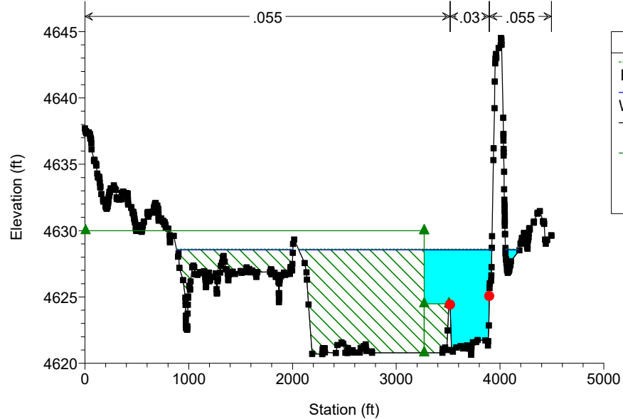
KCC-Lompa Ranch East_EOC Plan: KCC-Existing Geom: Existing Conditions Geometry Flow: FEMA Effective Flows River = KingsCynCreek Reach = Reach1 RS = 5179.23
