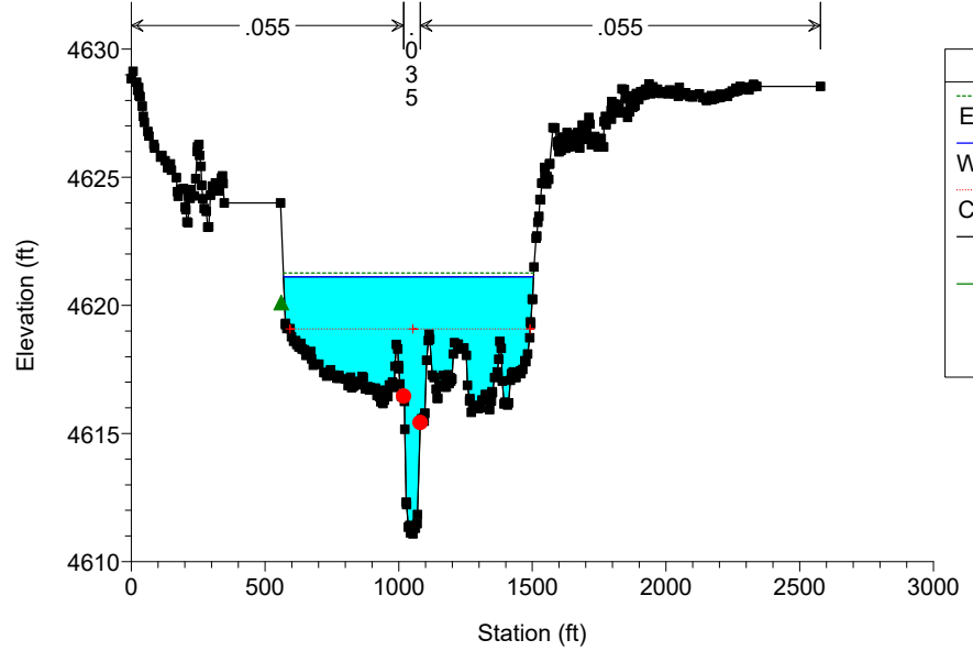
KCC-Lompa Ranch East_EOC Plan: KCC-Proposed Geom: Proposed Conditions Geometry Flow: FEMA Effective Flows River = KingsCynCreek Reach = Reach1 RS = 1137.728
