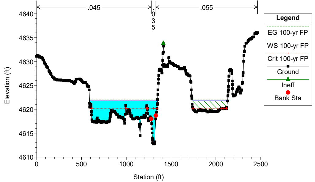
KCC-Lompa Ranch East_EOC Plan: KCC-Proposed Geom: Proposed Conditions Geometry Flow: FEMA Effective Flows River = KingsCynCreek Reach = Reach1 RS = 1552
