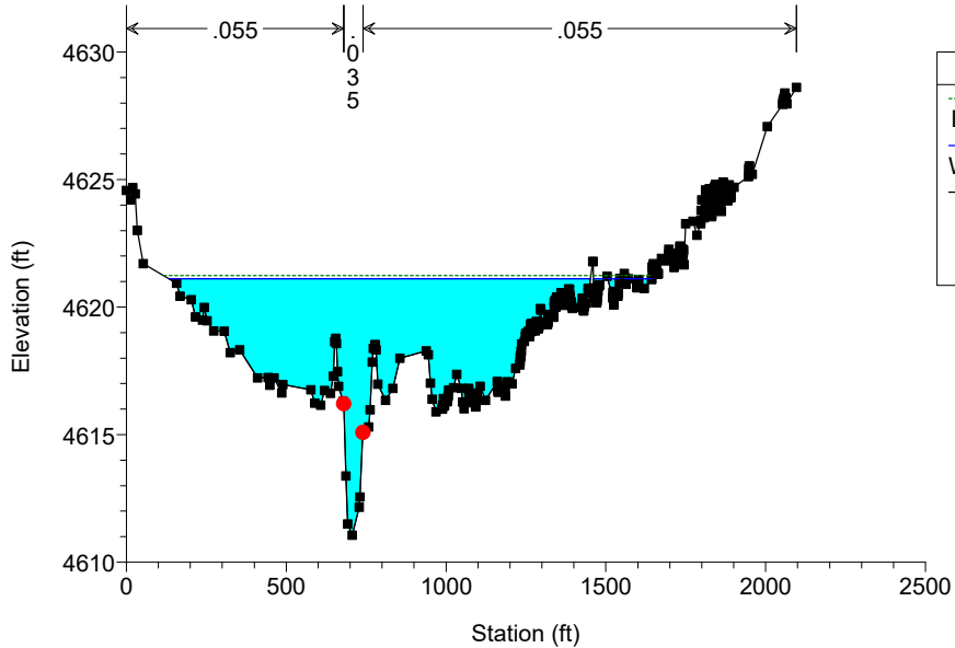
KCC-Lompa Ranch East_EOC Plan: KCC-Proposed Geom: Proposed Conditions Geometry Flow: FEMA Effective Flows River = KingsCynCreek Reach = Reach1 RS = 1212
