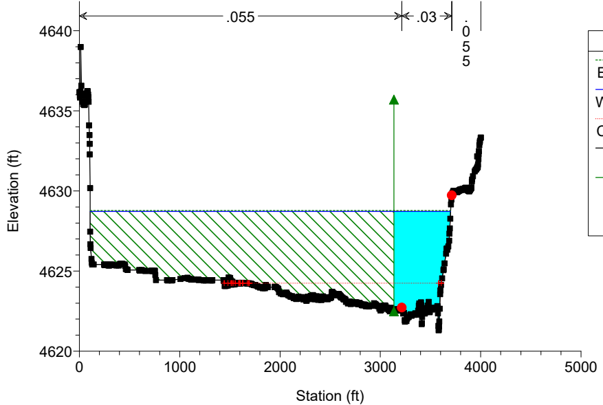
KCC-Lompa Ranch East_EOC Plan: KCC-Existing Geom: Existing Conditions Geometry Flow: FEMA Effective Flows River = KingsCynCreek Reach = Reach1 RS = 5489.854
